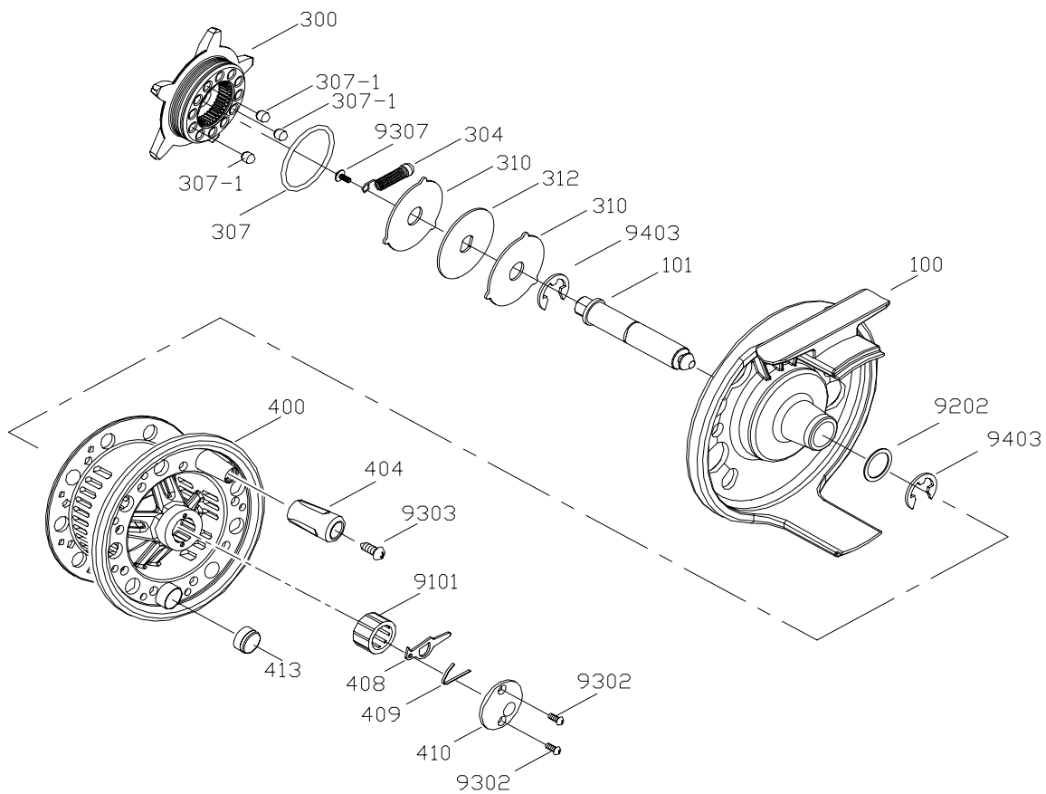
CW - 4/5/6 - PS6 Spare Parts
